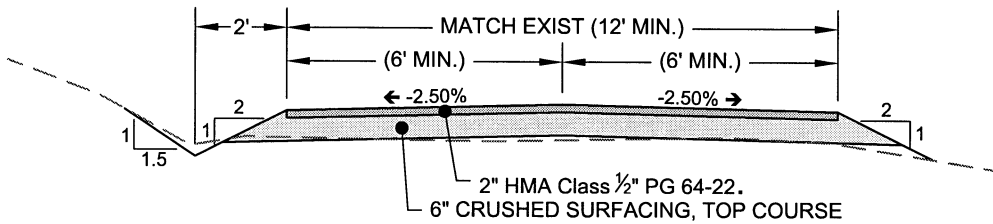
TYPICAL ASPHALT DRIVEWAY SECTION
