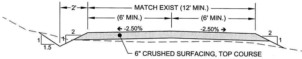
TYPICAL GRAVEL DRIVEWAY SECTION
