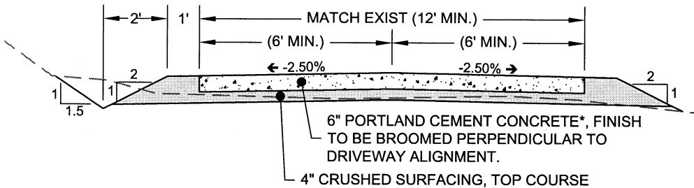
TYPICAL CONCRETE DRIVEWAY SECTION
