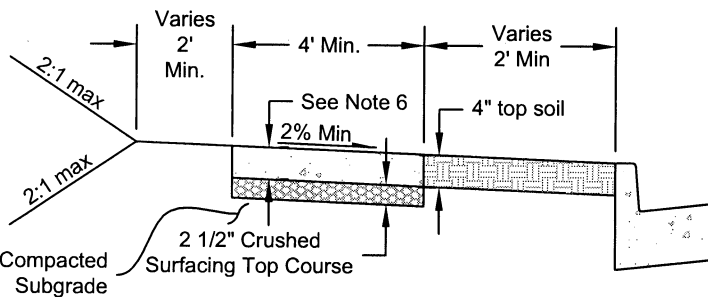
DETACHED SIDEWALK SECTION VIEW
