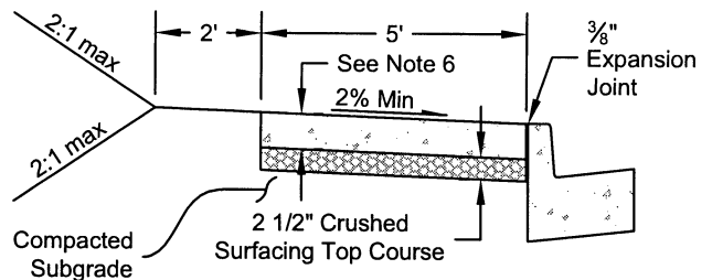
ATTACHED SIDEWALK SECTION VIEW
