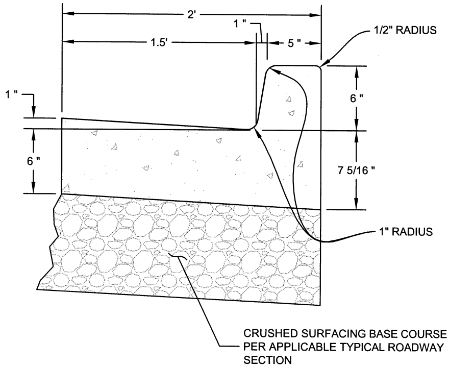
SECTION VIEW
